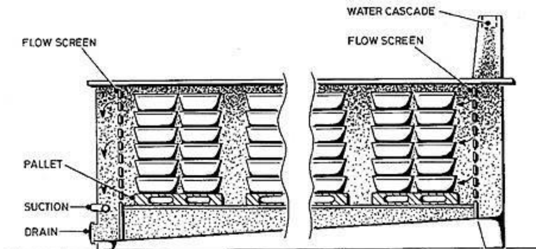
Side view of a multi-layer system
